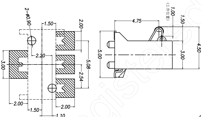
PCB LAYOUT
